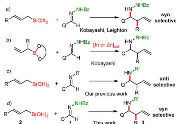
Figure 1. Stereoselective synthesis of homoallylamines.
