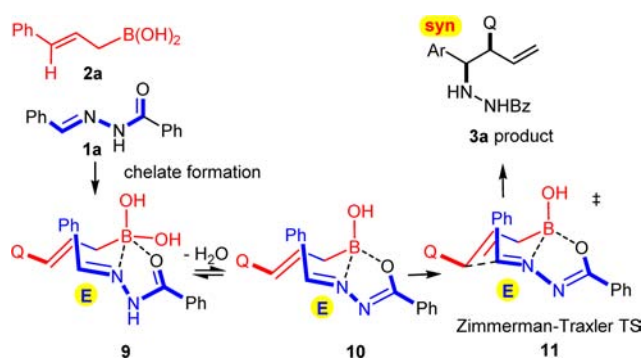
Figure 5. Syn selectivity in allylation of hydrazones.
