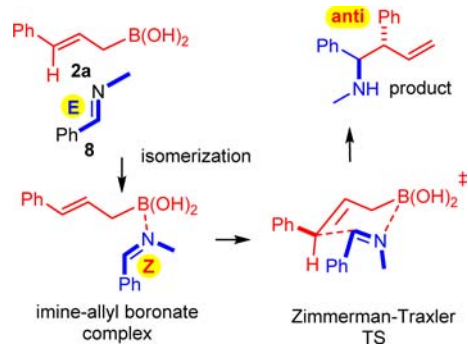
Figure 4. Anti selectivity in allylation of imines.
